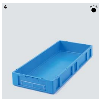
4 35 litres – Ref. 26S35* minimum order item Ext. dim.: L 800 x w 400 x h 140mm Ext. dim.: L 31.5 x w 15.7 x h 5.5" Int. dim.: L 761 x w 358 x h 127mm Int. dim.: L 30.0 x w 14.1 x h 5.0" Wt: 1.88 Kg/4.1 lbs., Colour: blue Label holder can be fitted to all 4 sides
