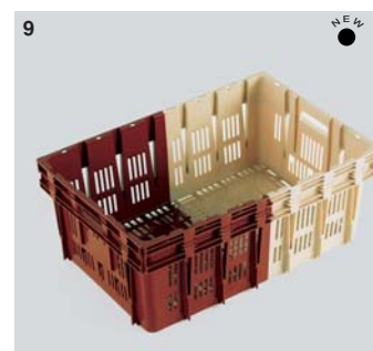
9 43 litres – Ref. AE218*** ventilated sides and base Ext. dim.: L 600 x w 400 x h 237mm Ext. dim.: L 23.6 x w 15.8 x h 9.3" Int. dim.: L 560 x w 360 x h 215mm Int. dim.: L 22.0 x w 14.2 x h 8.5" nested height: 69mm / 2.7" Wt: 1.75 Kg/3.6 lbs. Colour: brown-red/beige
