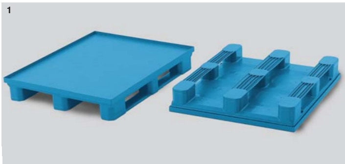
Ref. 3M300 pallet with 3 runners smooth deck Dim.: L 1,200 x w 1,000 x h 158mm Dim.: L 47.2 x w 39.4 x h 6.2" Weight: 23.5 Kg/51.7 lbs., Colour: blue Ref. 3M302 as ref. 3M300 with 7mm collar Dim.: L 1,200 x w 1,000 x h 165mm Dim.: L 47.2 x w 39.4 x h 6.5"
