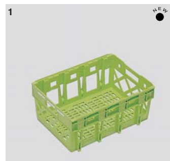
1 16 litres – Ref. EG150 minimum order item ventilated sides and base Ext. dim.: L 400 x w 300 x h 180mm Ext. dim.: L 15.8 x w 11.8 x h 7.1" Int. dim.: L 385 x w 258 x h 160mm Int. dim.: L 15.2 x w 10.2 x h 6.3" nested height: 63mm / 2.5" Wt: 0.9 Kg/2.0 lbs., Colour: green
