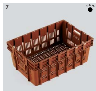
7 43 litres – Ref. AE216*** ventilated sides and base Ext. dim.: L 600 x w 400 x h 237mm Ext. dim.: L 23.6 x w 15.8 x h 9.3" Int. dim.: L 560 x w 360 x h 215mm Int. dim.: L 22.0 x w 14.2 x h 8.5" nested height: 69mm / 2.7" Wt: 2.00 Kg/4.4 lbs. Colour: brown-red
