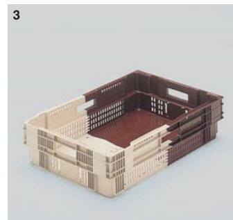
3 27 litres - Ref. 13A27* ventilated sides, drainage holes in base Ext. dim.: L 600 X w 400 X h 147 mm Ext. dim.: L 23.6 X w 15.8 X h 5.8" Int. dim.: L 553 X w 360 X h 131 mm Int. dim.: L 21.8 X w 14.2 X h 5.2" nested height: 76 mm/2.9" Wt: 1.54 kg/3.4 lbs. Colour: brown/beige. SKU quantity: 65
