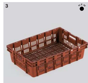
3 27 litres – Ref. AE136* ventilated sides and base Ext. dim.: L 600 x w 400 x h 155mm Ext. dim.: L 23.6 x w 15.8 x h 6.1" Int. dim.: L 560 x w 360 x h 135mm Int. dim.: L 22.0 x w 14.2 x h 5.3" nested height: 54mm / 2.1" Wt: 1.35 Kg/3.0 lbs. Colour: brown-red
