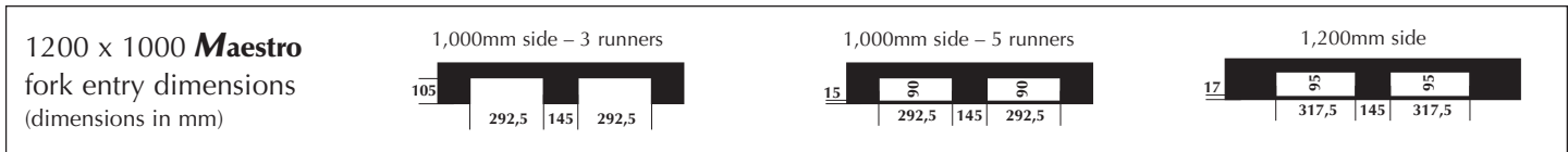
Ref. 3M500 pallet with 5 runners smooth deck Dim.: L 1,200 x w 1,000 x h 158mm Dim.: L 47.2 x w 39.4 x h 6.2" Weight: 24.2 Kg/53.2 lbs., Colour: blue 3 Ref. 3M502 as ref. 3M500 with 7mm collar Dim.: L 1,200 x w 1,000 x h 165mm Dim.: L 47.2 x w 39.4 x h 6.5"
