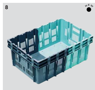
8 43 litres – Ref. AE217*** ventilated sides, drainage holes in base Ext. dim.: L 600 x w 400 x h 237mm Ext. dim.: L 23.6 x w 15.8 x h 9.3" Int. dim.: L 560 x w 360 x h 215mm Int. dim.: L 22.0 x w 14.2 x h 8.5" nested height: 69mm / 2.7" Wt: 1.86 Kg/4.1 lbs. Colour: grey/light grey
