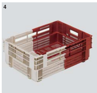
4 35 litres - Ref. 13034* ventilated sides and base with additional ventilation on sides Ext. dim.: L 600 X w 400 X h 187 mm Ext. dim.: L 23.6 X w 15.8 X h 7.4" Int. dim.: L 553 X w 360 X h 171 mm Int. dim.: L 21.8 X w 14.2 X h 6.7" nested height: 96 mm/3.7" Wt: 1.73 kg/3.8 lbs. Colour: brown-red/beige. SKU quantity: 50
