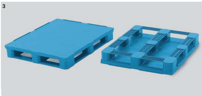
Ref. 3M500 pallet with 5 runners smooth deck Dim.: L 1,200 x w 1,000 x h 158mm Dim.: L 47.2 x w 39.4 x h 6.2" Weight: 24.2 Kg/53.2 lbs., Colour: blue 3 Ref. 3M502 as ref. 3M500 with 7mm collar Dim.: L 1,200 x w 1,000 x h 165mm Dim.: L 47.2 x w 39.4 x h 6.5"
