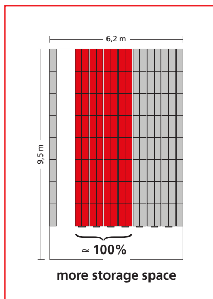
META MULTIBLOC® mobile shelving system
