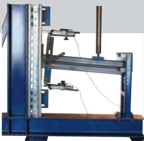
Beam connector under test in the META- laboratory: End of test
