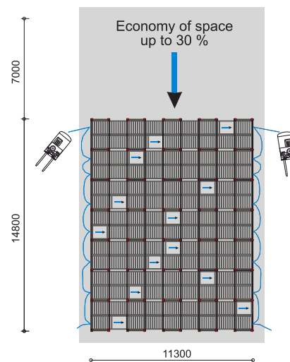
Driveway in a META MULTILINE® S Flow rack
