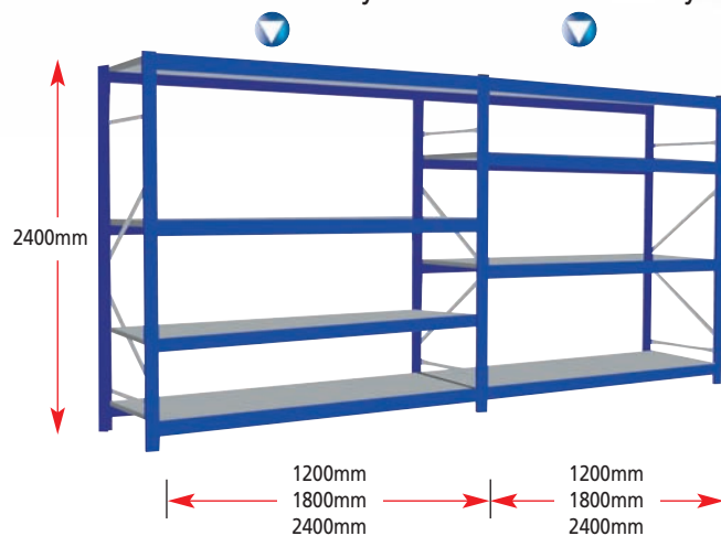
4-Beam Starter Bay
