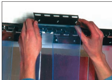
Medium duty hook-on track (overlap is slightly reduced with this track)
