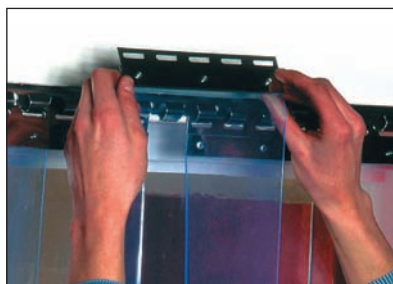
Medium duty hook-on track (overlap is slightly reduced with this track)
