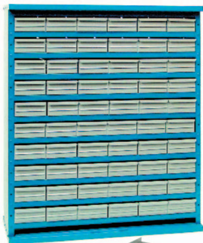
Drawer W x H: 135 x 75mm Drawer D: 285 or 440mm Divider slots at 20mm centres
